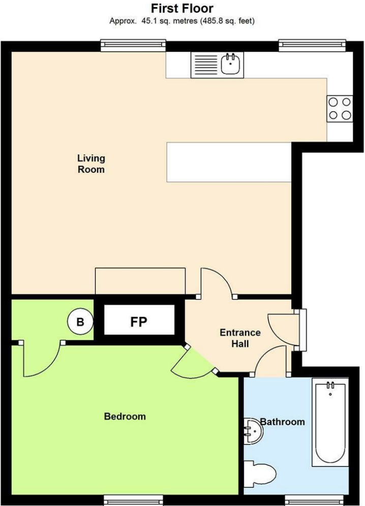
Total area: approx. 45.1 sq. metres (485.8 sq. feet) Flat 2, Barrows House, The Street, Borden, Sittingbourne
